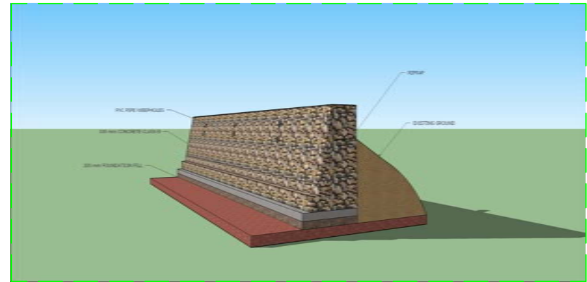
CONSTRUCTION OF RIPRAP AT LEAST 280 l.m. LENGTH
